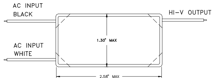
BOTTOM VIEW
